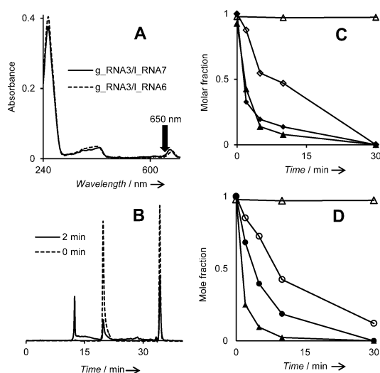
Figure 5. A) UV/Vis spectra of g_RNA3/l_RNA6 (1 μM) and g_RNA3/l_RNA7 (1 μM) in phosphate buffer (20 mM, pH 7.4, NaCl 130 mM), 22 °C. B) HPLC profiles of g_RNA3/l_RNA6 (50 μM) obtained before (dotted trace) and after uncaging with 650 nm light for 2 min (0.23 W, solid trace). The peak observed at 34.2 min corresponds to l_RNA6, that at 19.7 min to g_RNA3 and that at 12.4 min to g_RNA2. C) Kinetics of uncaging of g_RNA3 in g_RNA3/l_RNA9 (open triangles) and g_RNA3/l_RNA7 (black triangles) and of photobleaching of l_RNA7 in g_RNA2/l_RNA7 (open diamonds) and g_RNA3/l_RNA7 (black diamonds); molar fraction of g_RNA3 = [g\_RNA3]/([g\_RNA3] + [g\_RNA2]) ; molar fraction of l_RNA7 = [l\_RNA7]/([l\_RNA7] + [l\_RNA6]) . D) Kinetics of uncaging of g_RNA3 in g_RNA3/l_RNA9 (open triangles) and g_RNA3/l_RNA6 (black triangles) and of photobleaching of l_RNA6 in g_RNA2/l_RNA6 (open circles) and g_RNA3/l_RNA6 (black circles); molar fraction of l_RNA6 = [l\_RNA6]/([l\_RNA6] + [l\_RNA7]) .
